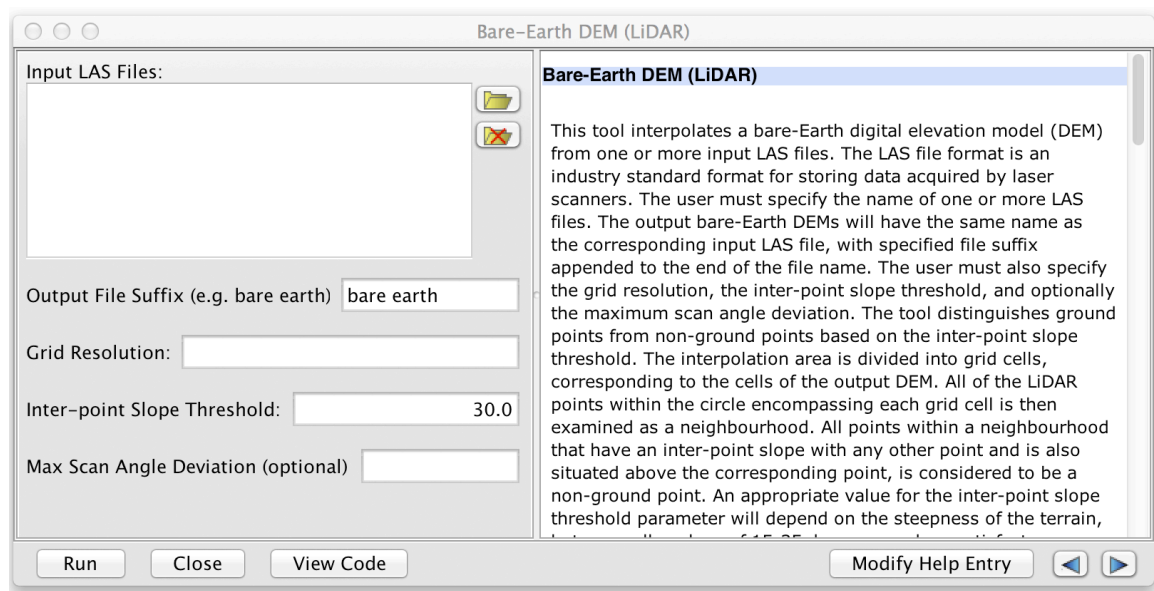
Figure 2. A typical tool dialog box including input parameters box, integrated help, and the 'View Code' button that is central to the concept of open-access software.
